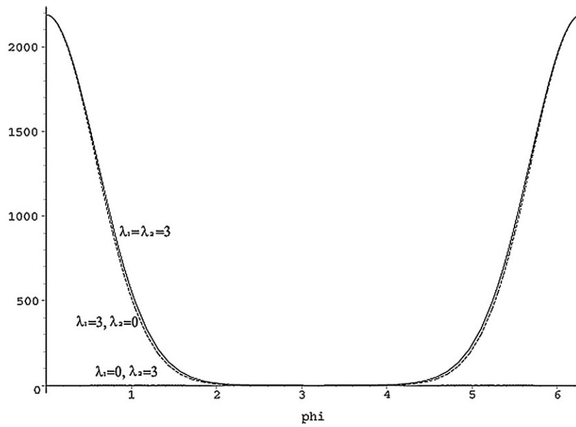
Figure 9. A plot of |I_2I(2\lambda_1 \cos(\frac{\phi}{2}) + i2\lambda_2 \sin(\frac{\phi}{2}))|^2 in terms of \phi , for some different values of \lambda_1 and \lambda_2 .
