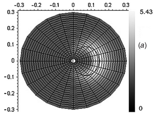
Figure 1. A plot of probability density |\Psi_N(r, \phi)|^2 for N = 7 (i.e., 2 \leq l \leq 9 ), \theta_o = 0 , A = 1 , \epsilon = 0 (i.e., the V(r, \phi) is real) and \lambda = 0.0 . This is the localized state corresponding to the classical trajectory of a particle which experiences just the first term of the potential, i.e. V(r, \phi) = -\Gamma/r^4 and therefore it is the reference plot.
