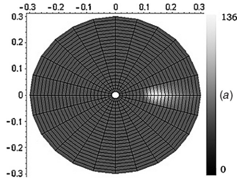
Figure 7. A plot of probability density |\Psi_N(r, \phi)|^2 for N = 7 (i.e., 2 \leq l \leq 9 ), \theta_o = 0 , A = 1 , \lambda = 100 .
