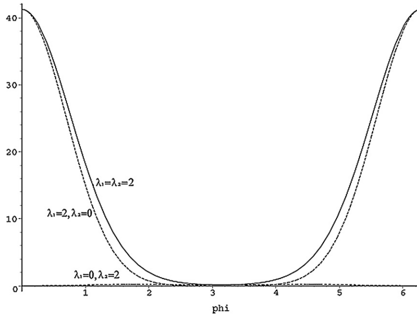
Figure 8. A plot of |I_2I(2\lambda_1 \cos(\frac{\phi}{2}) + i2\lambda_2 \sin(\frac{\phi}{2}))|^2 in terms of \phi , for some different values of \lambda_1 and \lambda_2 .
