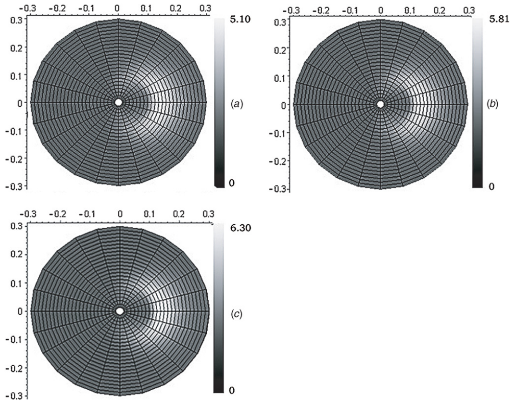
Figure 4. A plot of probability density |\Psi_N(r, \phi)|^2 for N = 7 (i.e., 2 \leq l \leq 9 ), \theta_0 = 0 , A = 1 , \lambda = 1 . Also (a), (b) and (c) are correspondence with V(r, \phi) = V_-, V_+ and V_c , respectively.
