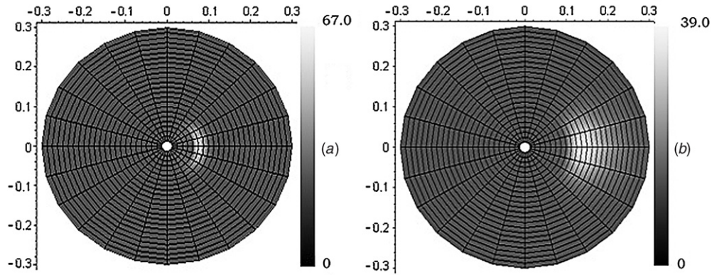
Figure 6. A plot of probability density |\Psi_N(r, \phi)|^2 for N = 7 (i.e., 2 \leq l \leq 9 ), \theta_o = 0 , A = 1 , \lambda = 10 . Also (a) and (b) are correspondence with V(r, \phi) = V_+ and V_c , respectively.
