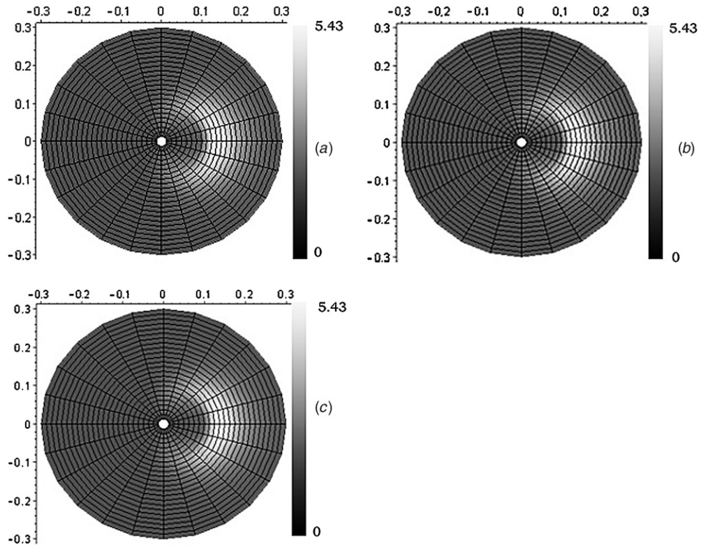
Figure 2. A plot of probability density |\Psi_N(r, \phi)|^2 for N = 7 (i.e., 2 \leq l \leq 9 ), \theta_o = 0 , A = 1 , \lambda = 0.1 . Also (a), (b) and (c) are correspondence with V(r, \phi) = V_-, V_+ and V_c , respectively.
