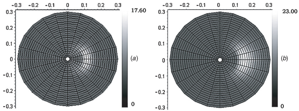
Figure 5. A plot of probability density |\Psi_N(r, \phi)|^2 for N = 7 (i.e., 2 \leq l \leq 9 ), \theta_0 = 0 , A = 1 , \lambda = 5 . Also (a) and (b) are correspondence with V(r, \phi) = V_+ and V_c , respectively.
