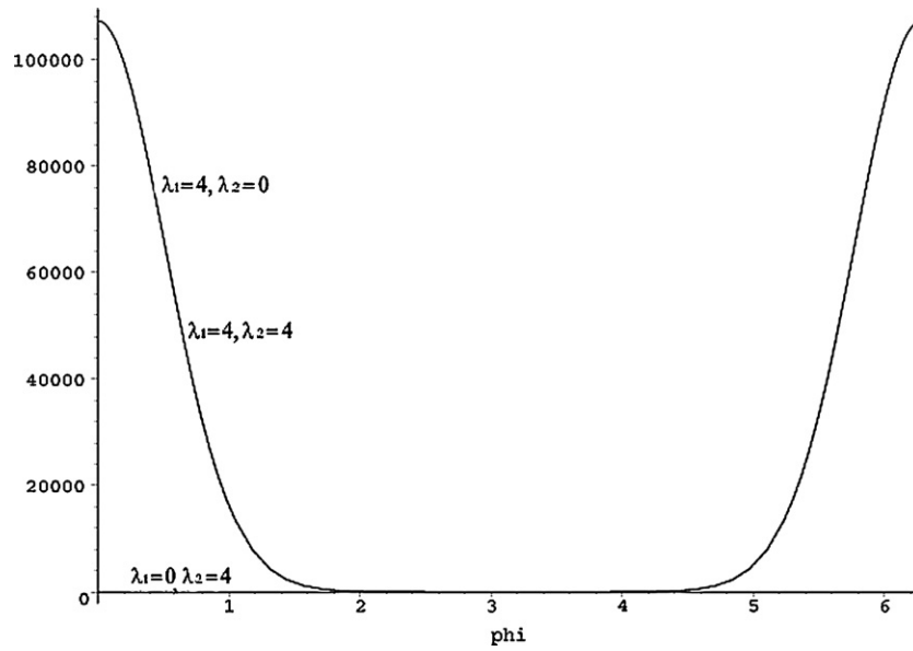
Figure 10. A plot of |I_{2l}(2\lambda_1 \cos(\frac{\phi}{2}) + i2\lambda_2 \sin(\frac{\phi}{2}))|^2 in terms of \phi , for some different values of \lambda_1 and \lambda_2 .
