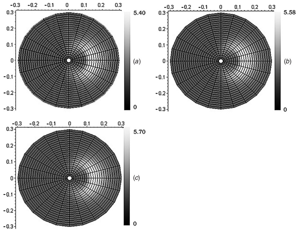
Figure 3. A plot of probability density |\Psi_N(r, \phi)|^2 for N = 7 (i.e., 2 \leq l \leq 9 ), \theta_o = 0 , A = 1 , \lambda = 0.5 . Also (a), (b) and (c) are correspondence with V(r, \phi) = V_-, V_+ and V_c , respectively.
